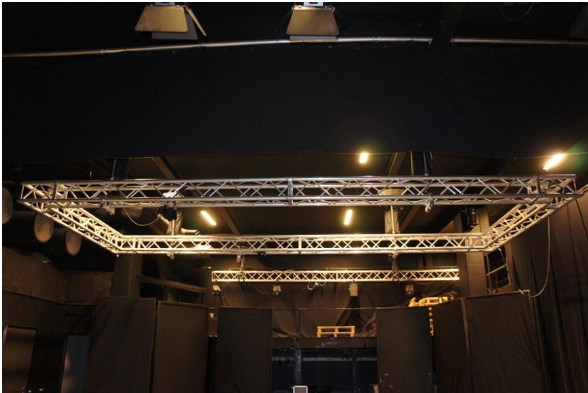
Truss 3 & 4.
